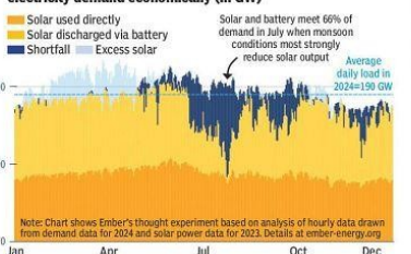
Solar plus battery could supply 90% of national electricity demand economically (in GW)
